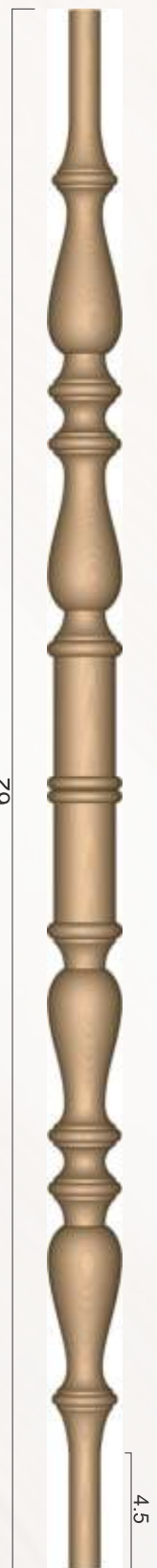
BR311 3x62 ends 1.25 dia.
